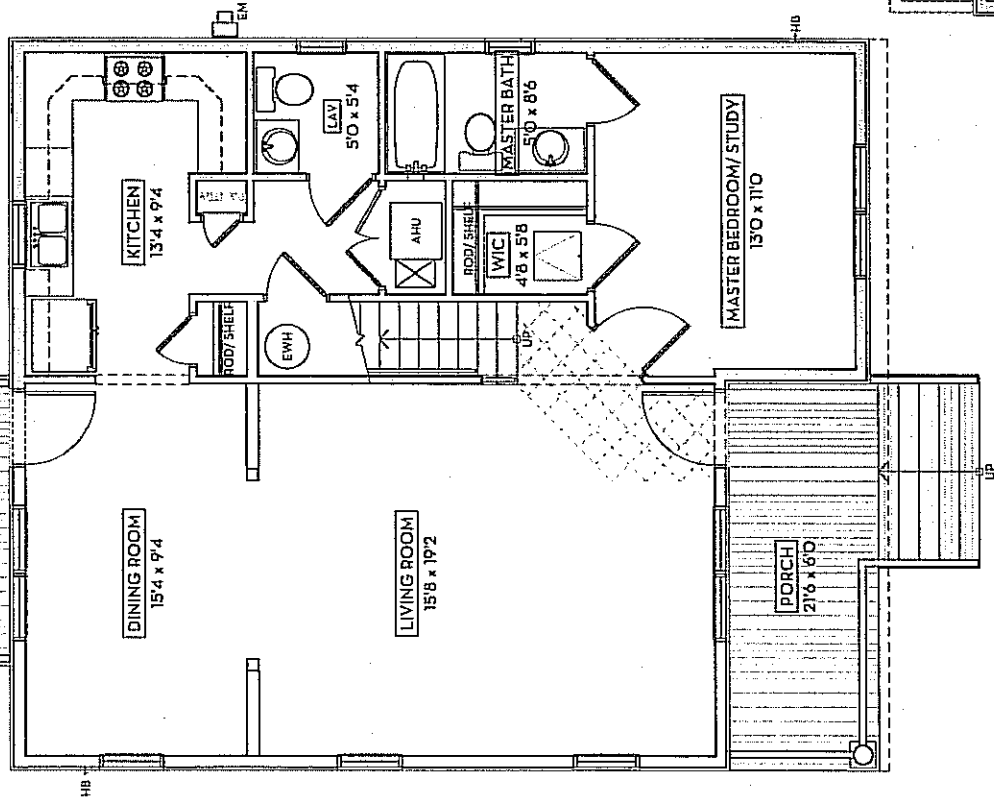
FIRST FLOOR PLAN 1/8" = 1'-0"
