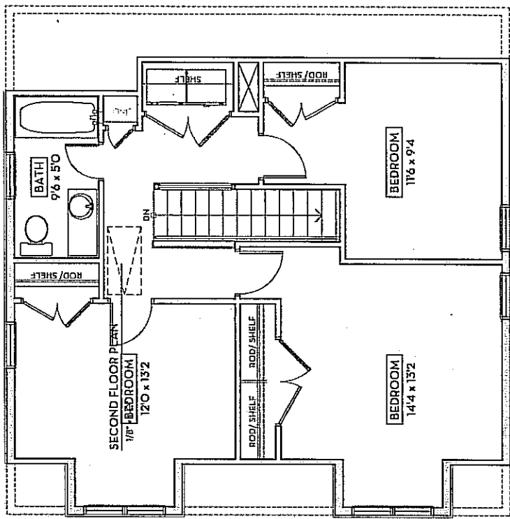
SECOND FLOOR PLAN 1/8" = 1'-0"
